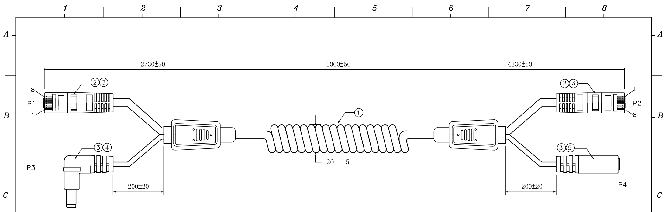
Wiring Diagram
