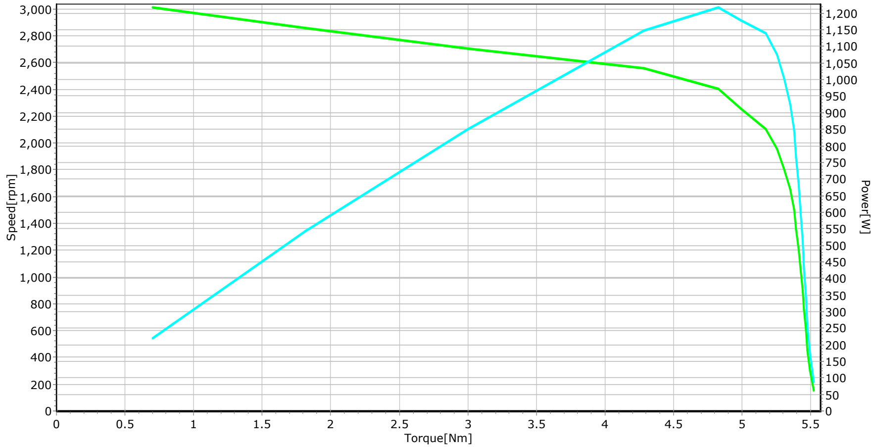
Speed,Power v. Torque
