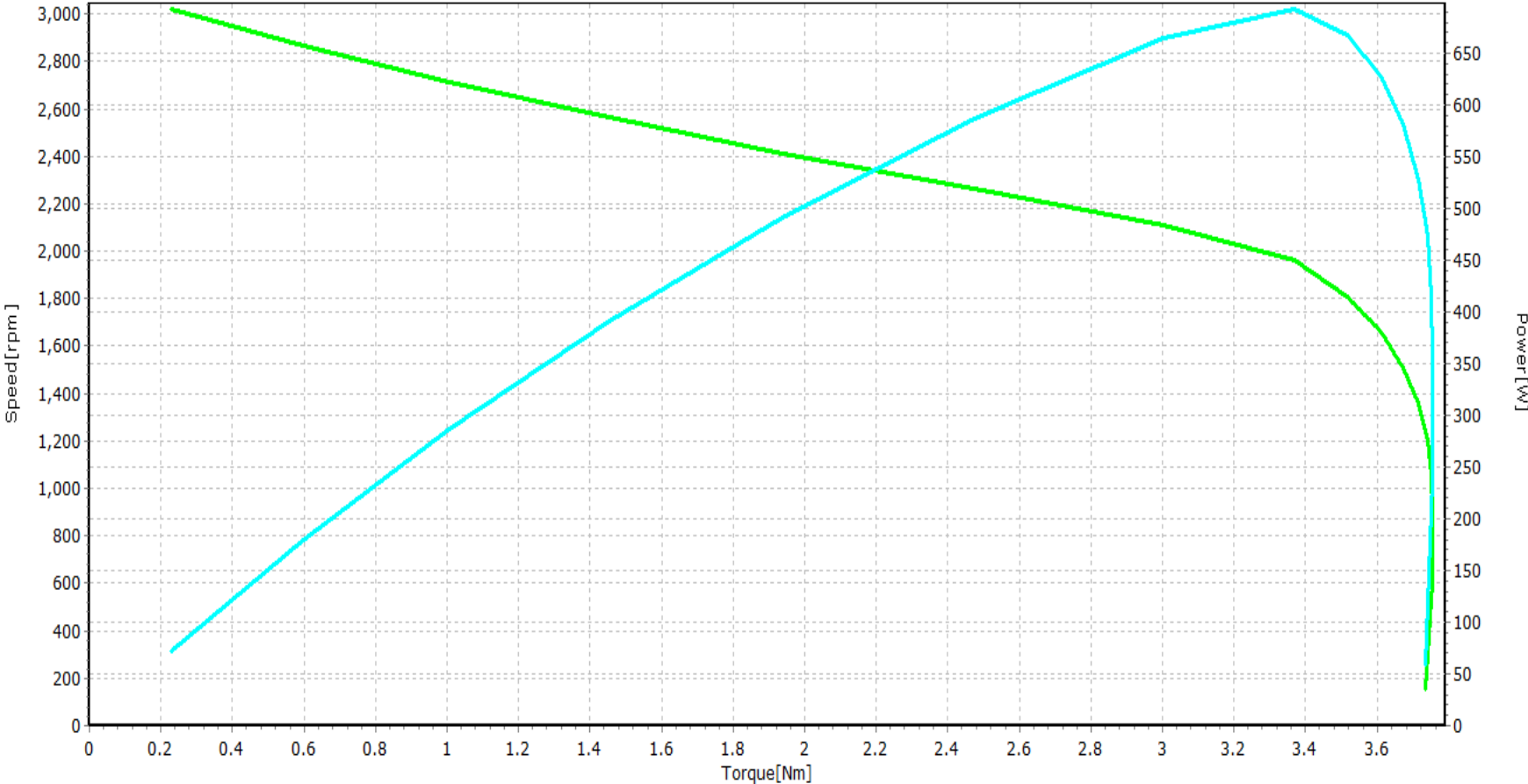
Speed,Power v. Torque
