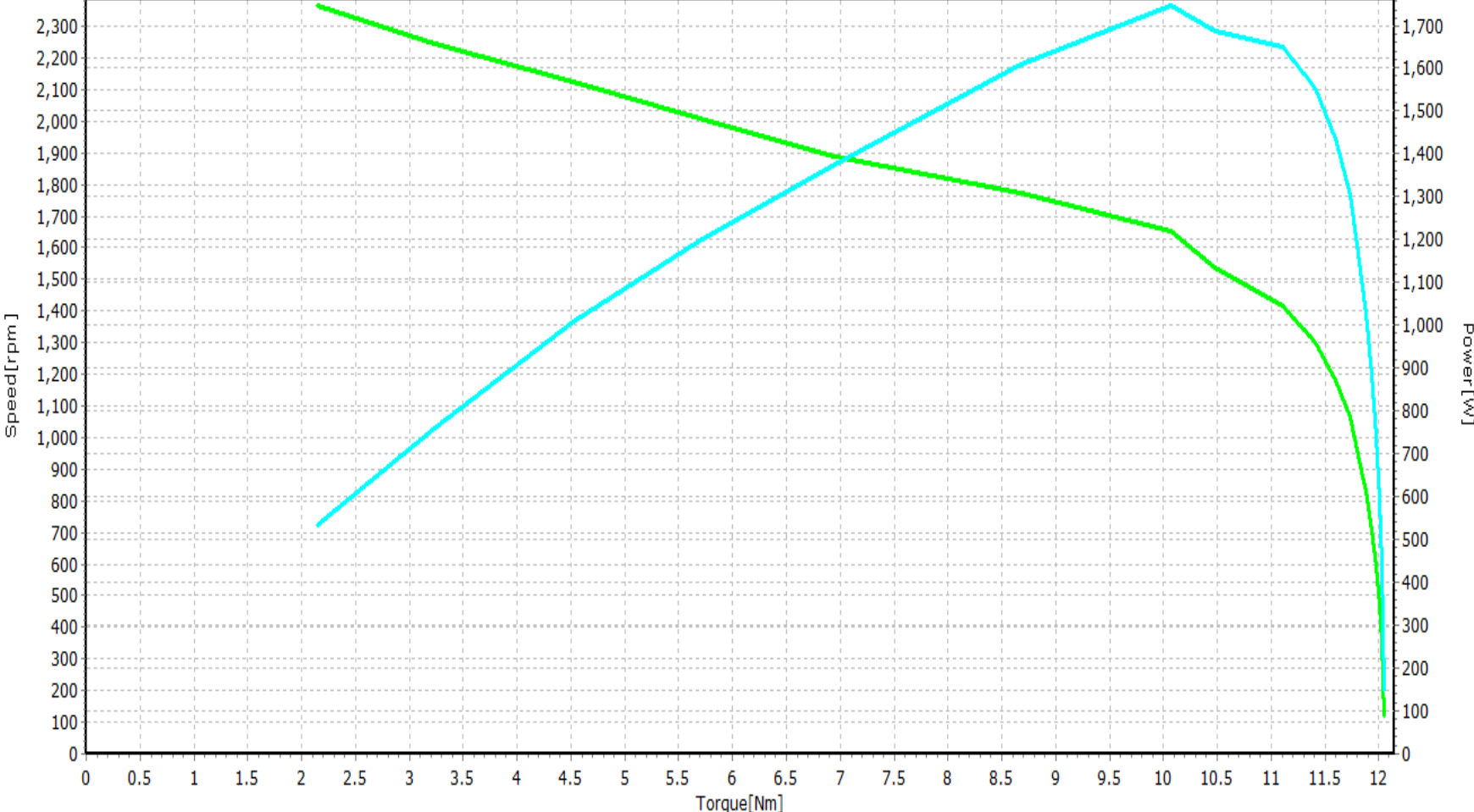
Speed,Power v. Torque
