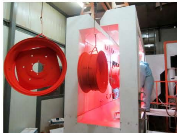
Powder coating for wheel
